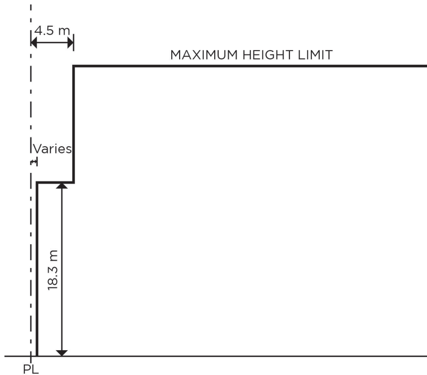
Figure 3 Height Limit at North/South Lane between 2nd and 5th Avenue
